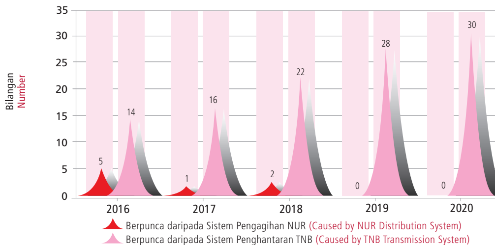
Carta 14: Kejadian Junaman Voltan yang Dilaporkan di Kulim Hi-Tech Park (KHTP) Chart 14: Voltage Dips Incidents Reported in Kulim Hi-Tech Park (KHTP)
