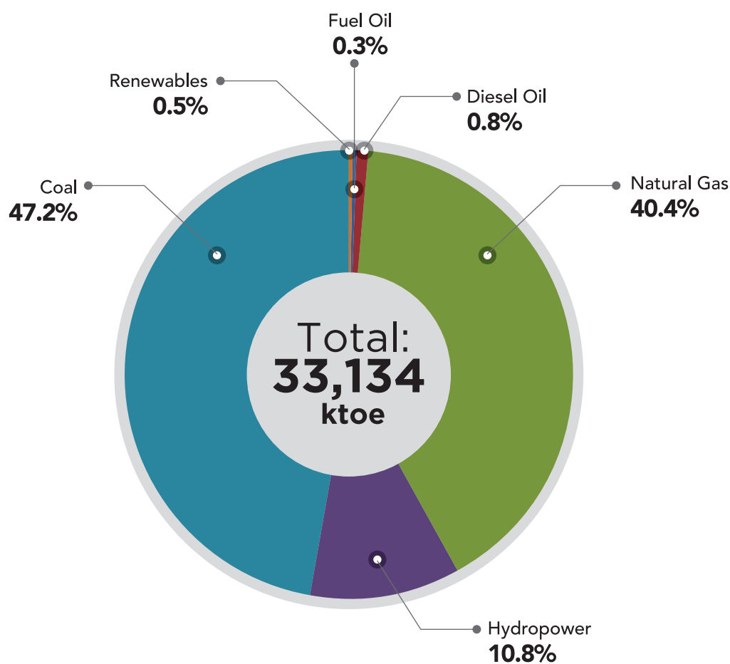
Figure 29: Energy Input in Power Stations
